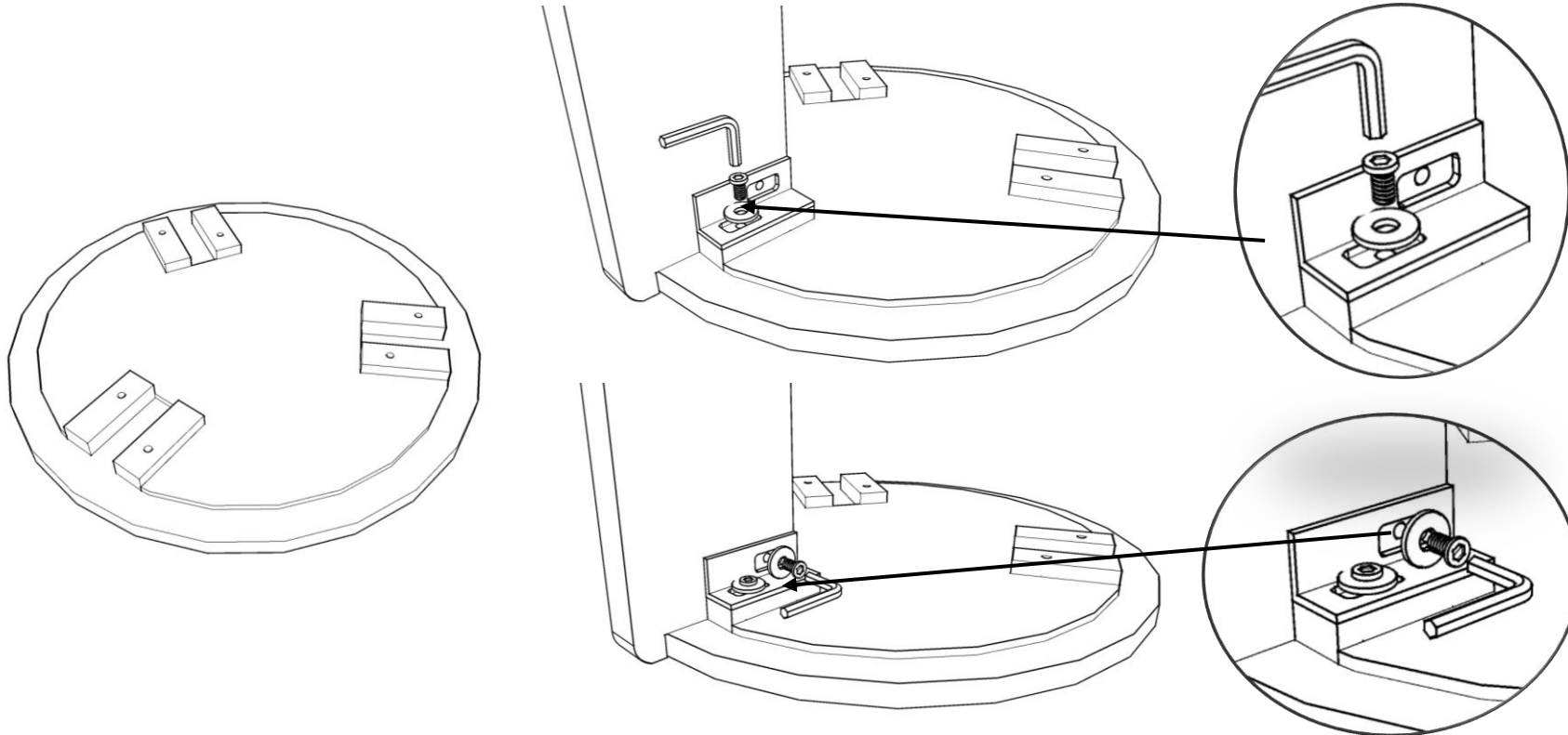
METAL CLIP – 6 PCs
